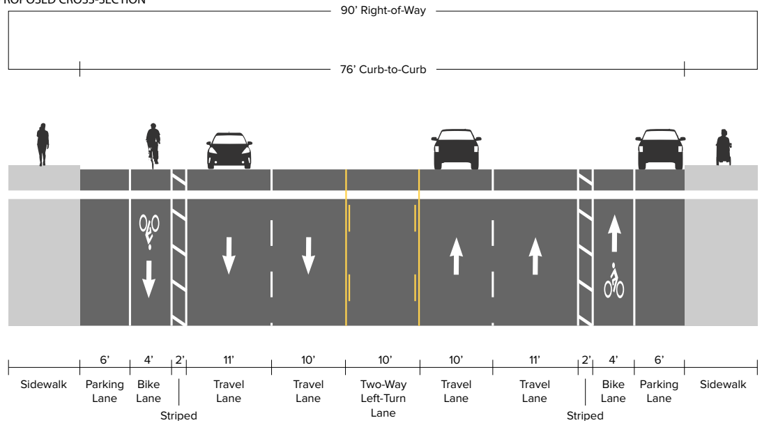
ARROW HWY: INDIAN HILL BLVD TO SPRING ST PROPOSED CROSS-SECTION
